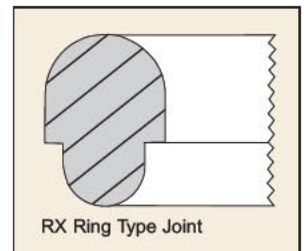
Transition RTJ
