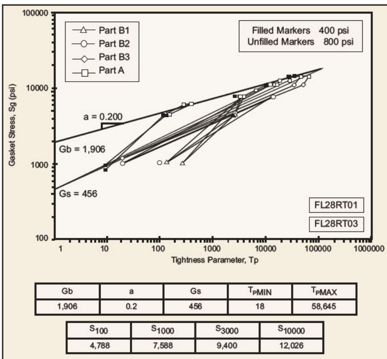
Room Temperature Tightness (ROTT) behavior characterization (Refer to page 48 for new method for determining factors.)
