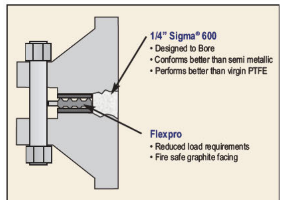
Resist further corrosion
