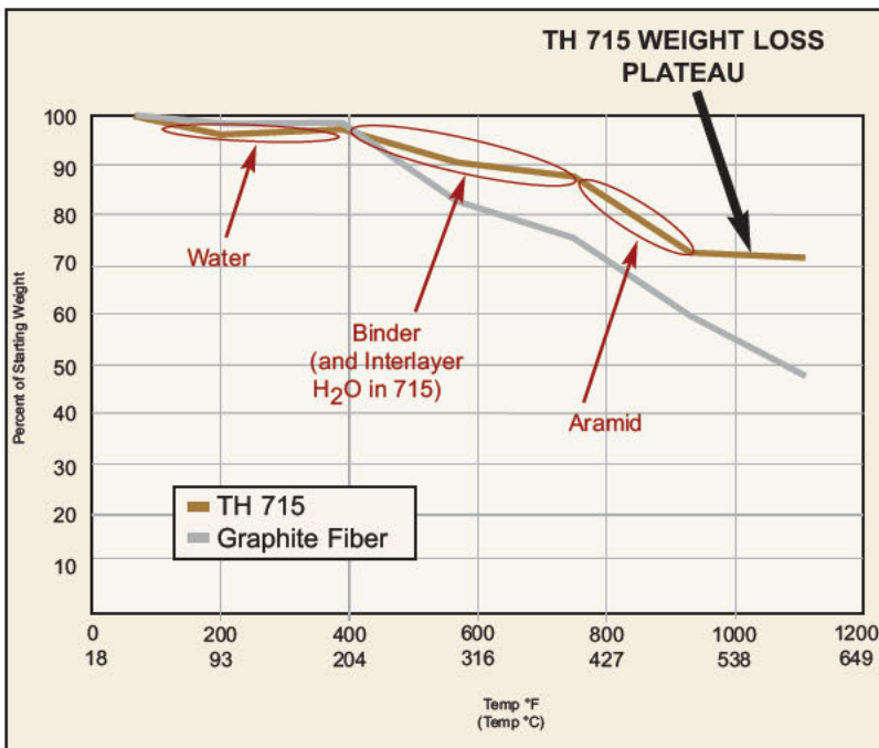
TGA, Thermiculite® 715 vs. Graphite Fiber - Graph shows a Thermogravimetric Analysis of TH 715 versus a well known and commonly used graphite fiber sheet. A TGA measures weight loss after exposure to air at elevated temperatures.
