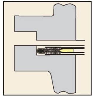
Carrier Ring
