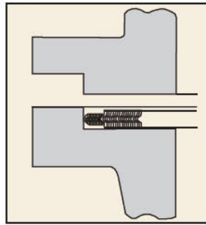
Style CG-RJ
