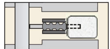
Eliminate crevices to prevent the onset of corrosion. Inner ring will not fall out.
