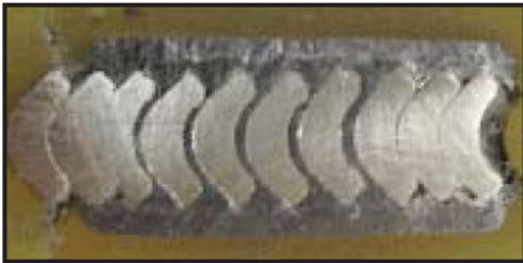
Wound like a spiral. Faced like a kammprofile.
