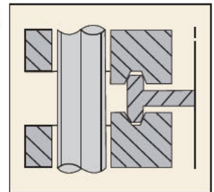
Blind RTJ
