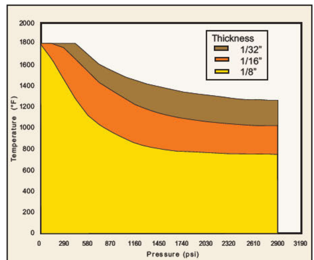
Flexitallic Thermiculite® 815 Pressure/Temperature Curve
